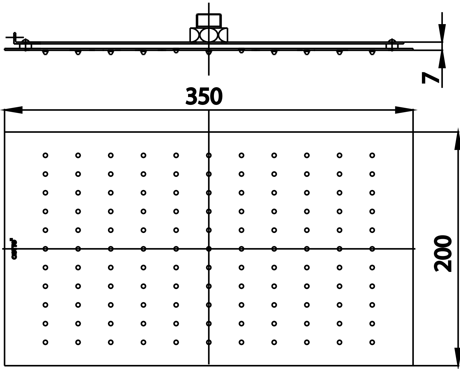
RAIN CENTER PLATE ZF01RC
