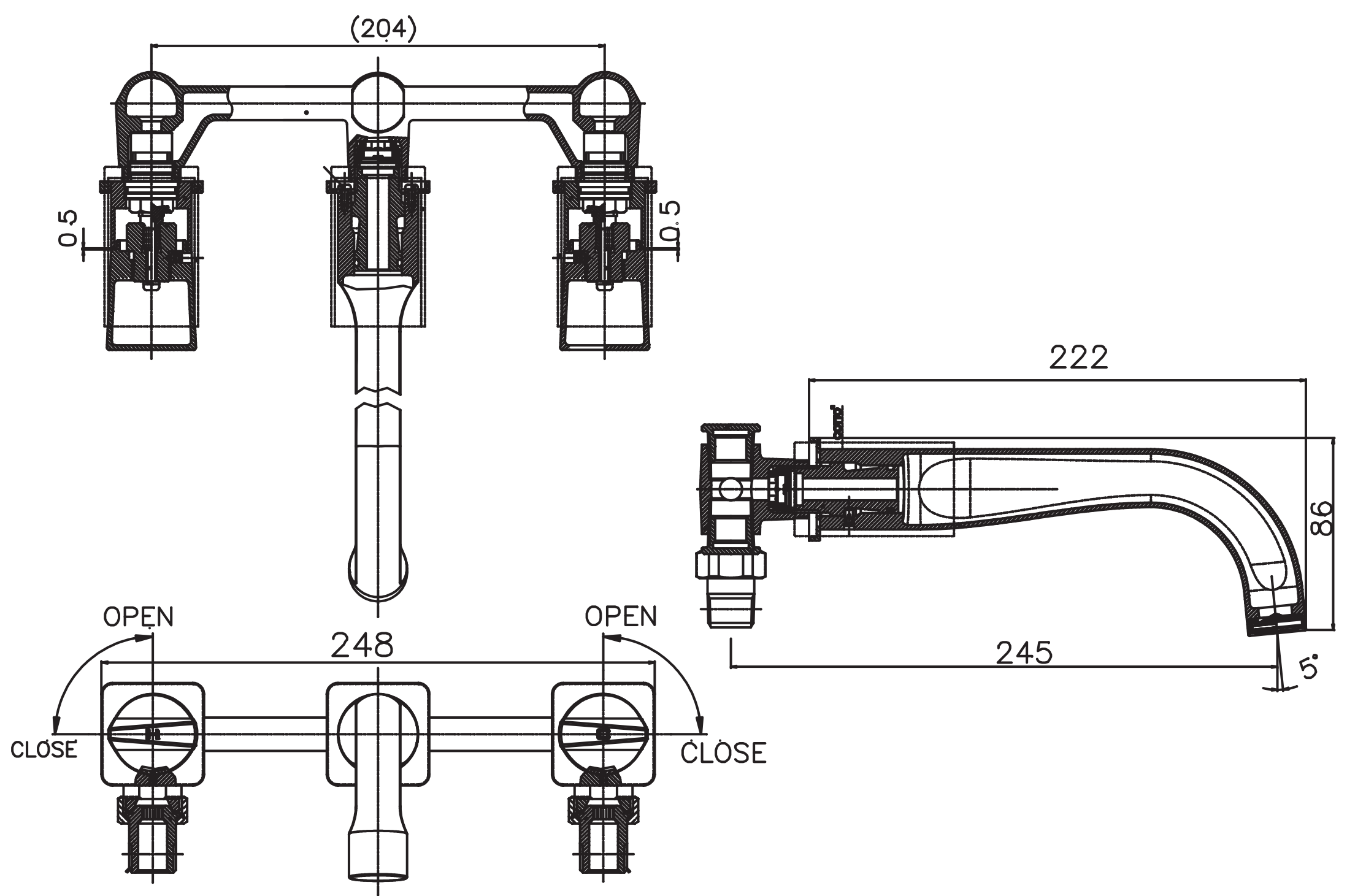
3 Holes Basin Mixer Wall Mounted CT 2 2 8 3
