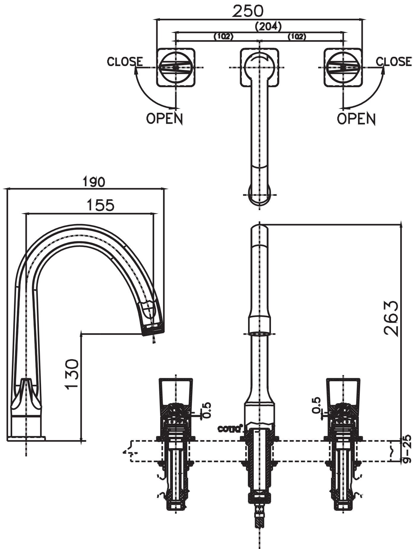
3 Holes Basin Mixer Deck Mounted C T 2 2 8 2
