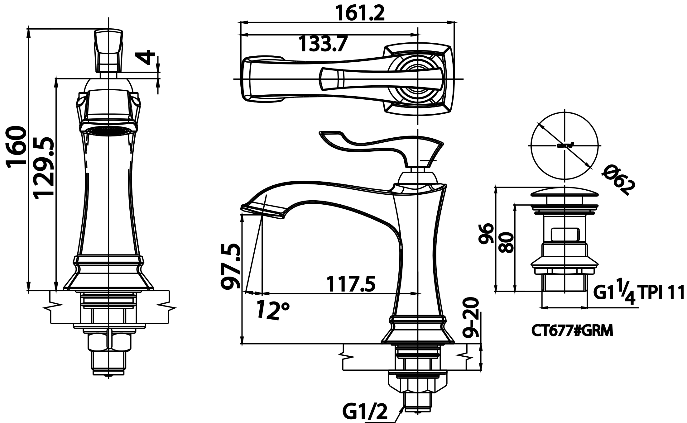
BASIN FAUCET CT1202A#GRM
