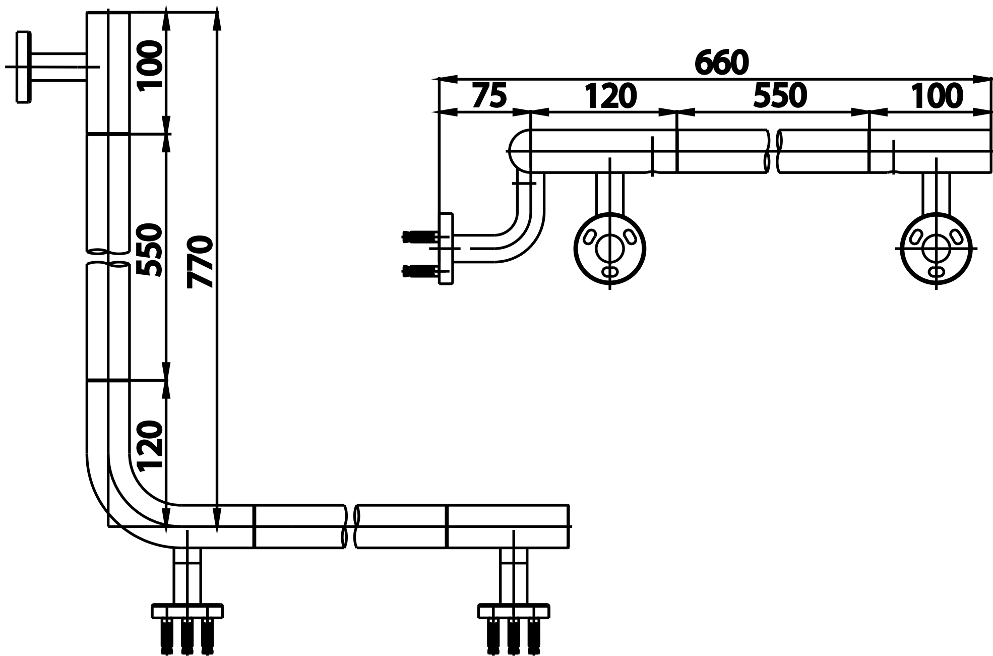
INSIDE CORNER HANDRAIL 150CM CT0202
