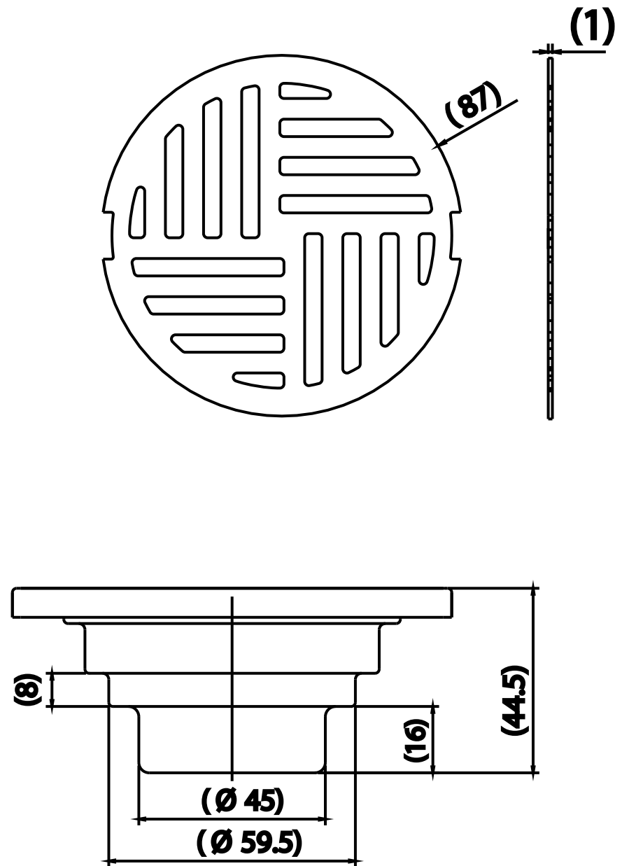
STAINLESS FLOOR DRAIN/SQUARE BODY CTSE6403Z1PW
