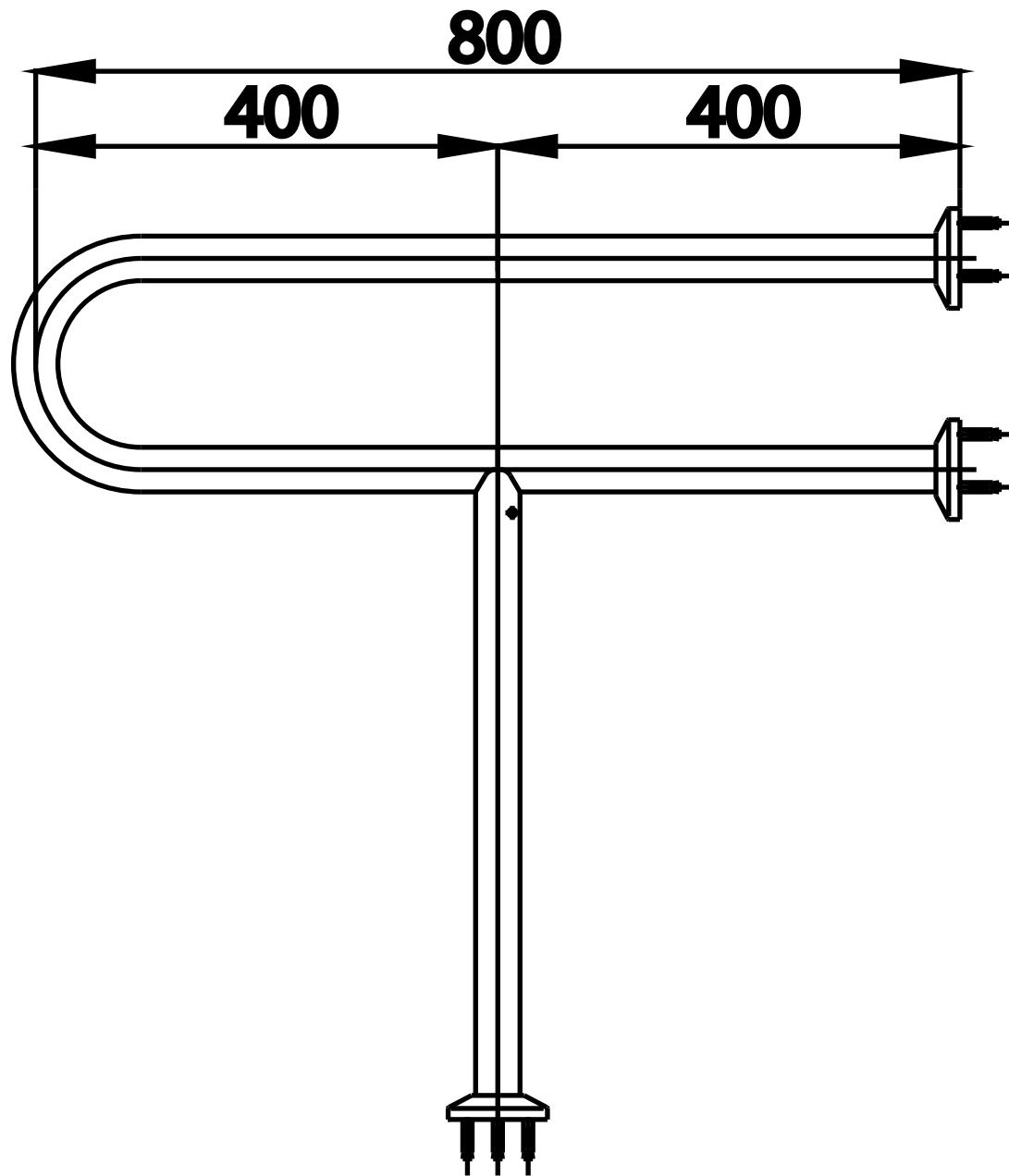
HAND RAIL FOR LAVATORY CT795
