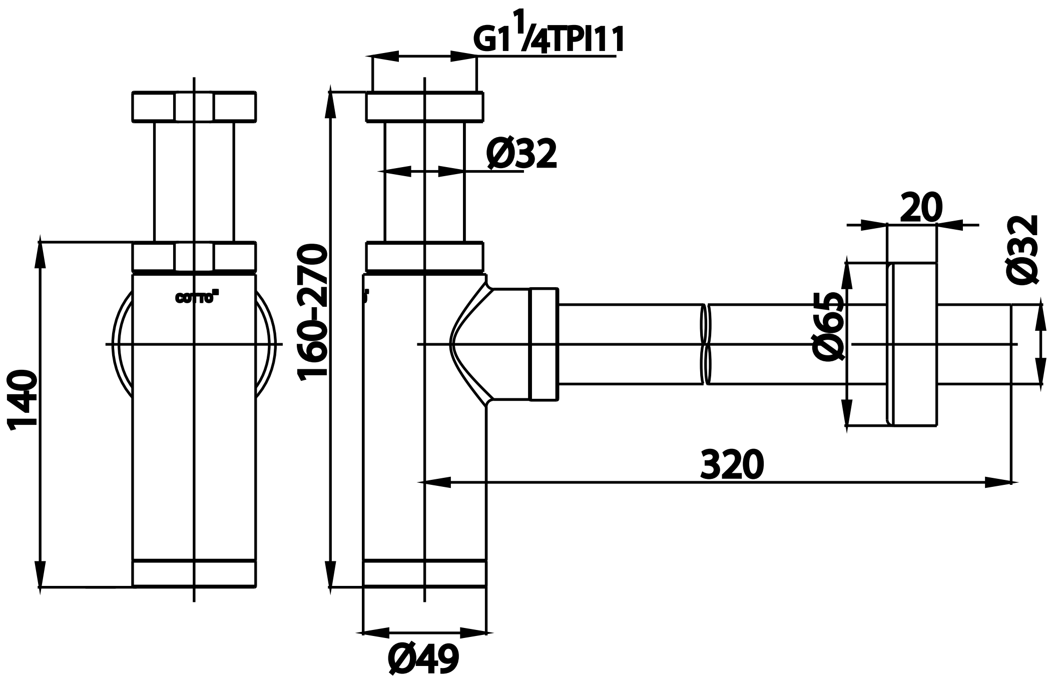
32 CM. BASIN TRAP CYLINDER SHAPE CT685 N(HM)
