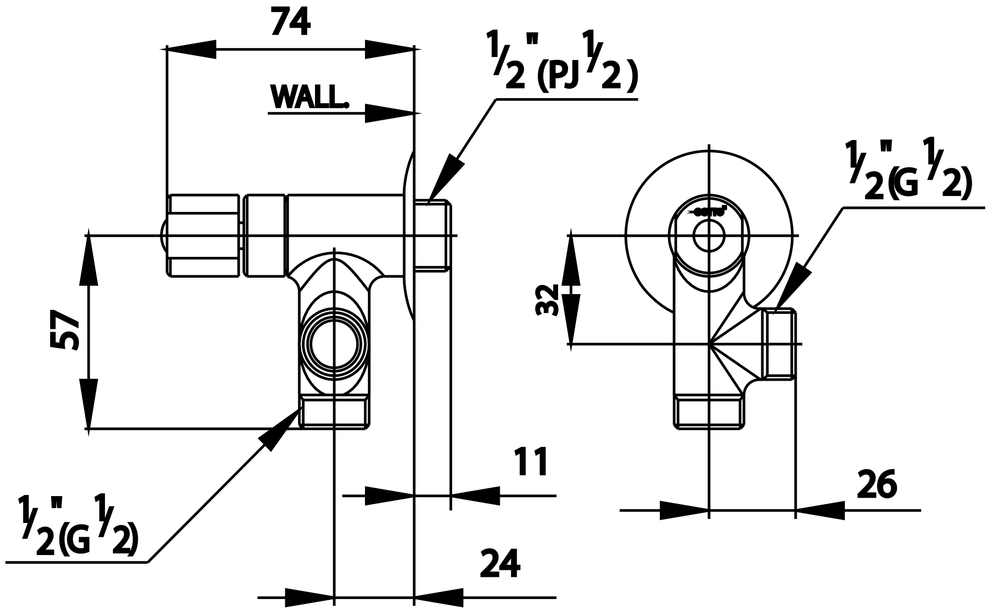
STOP VALVE CT 128 (HM)
