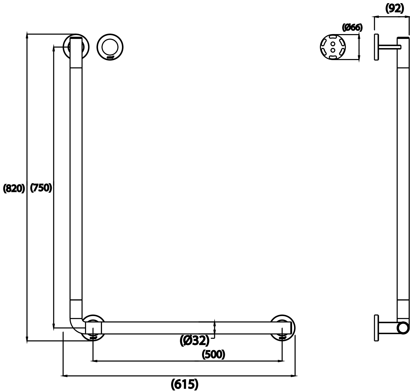
L-SHAPE HANDRAIL 50x75 CM CT0379 #SA(R), #GG(R), #BGR(R)
